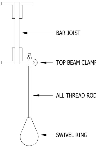
FIRE SUPPRESSION HANGER DETAIL NOT TO SCALE
