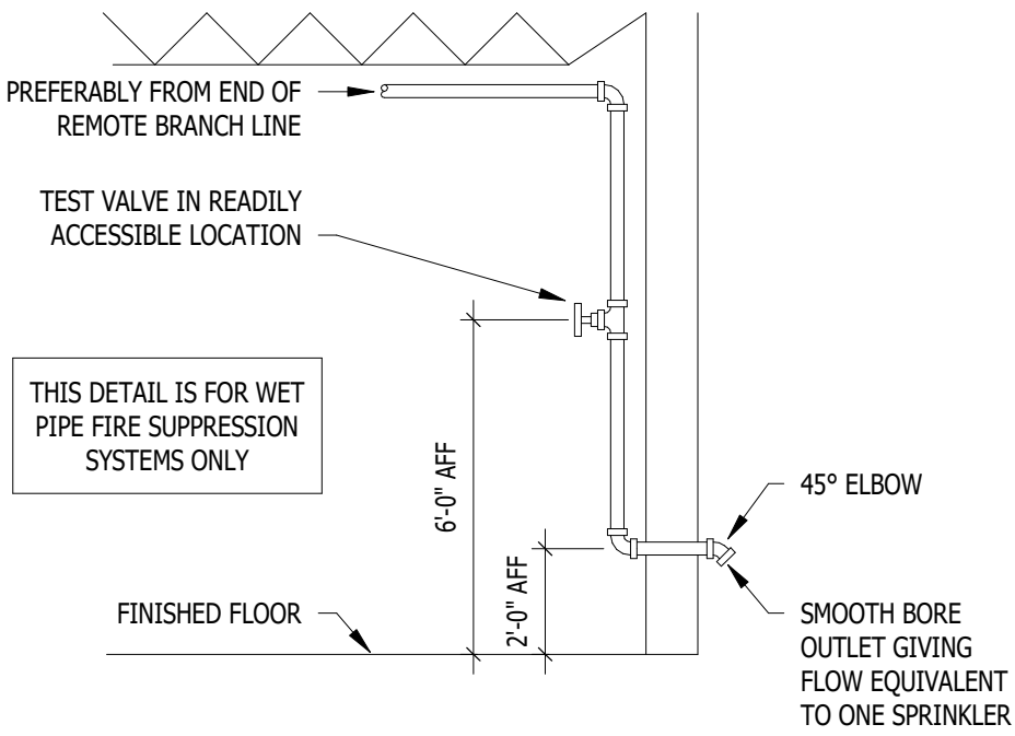
SYSTEM TEST CONNECTION DETAIL NOT TO SCALE
