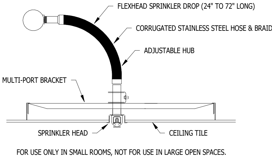
FIRE SUPPRESSION FLEXHEAD DETAIL NOT TO SCALE
